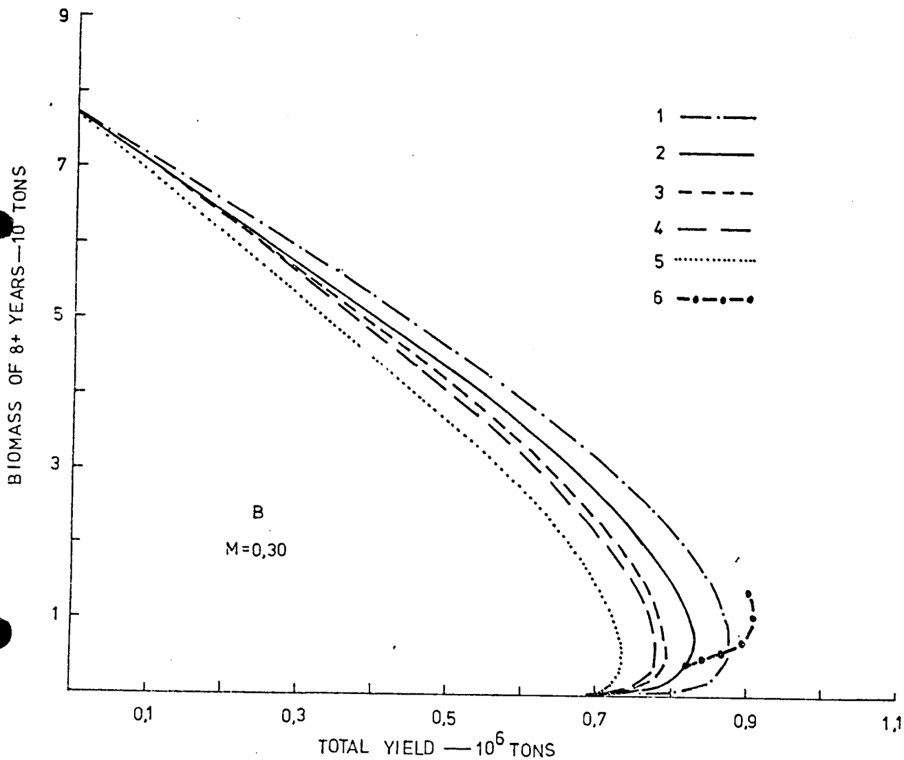
Fig. 4 B. The curves 1 to 5 show the size of the mature stock, measured by the biomass of fish 8 year old and older, as function of the total yield by different fishing patterns. Legend as in Fig.1. Curve 6 shows the relation between the total yield and the size of the mature stock when the mesh sizes in the total trawl fishery is increased from 120 mm to 230 mm, while the effort is kept constant at the 1970 - 1974 level.
